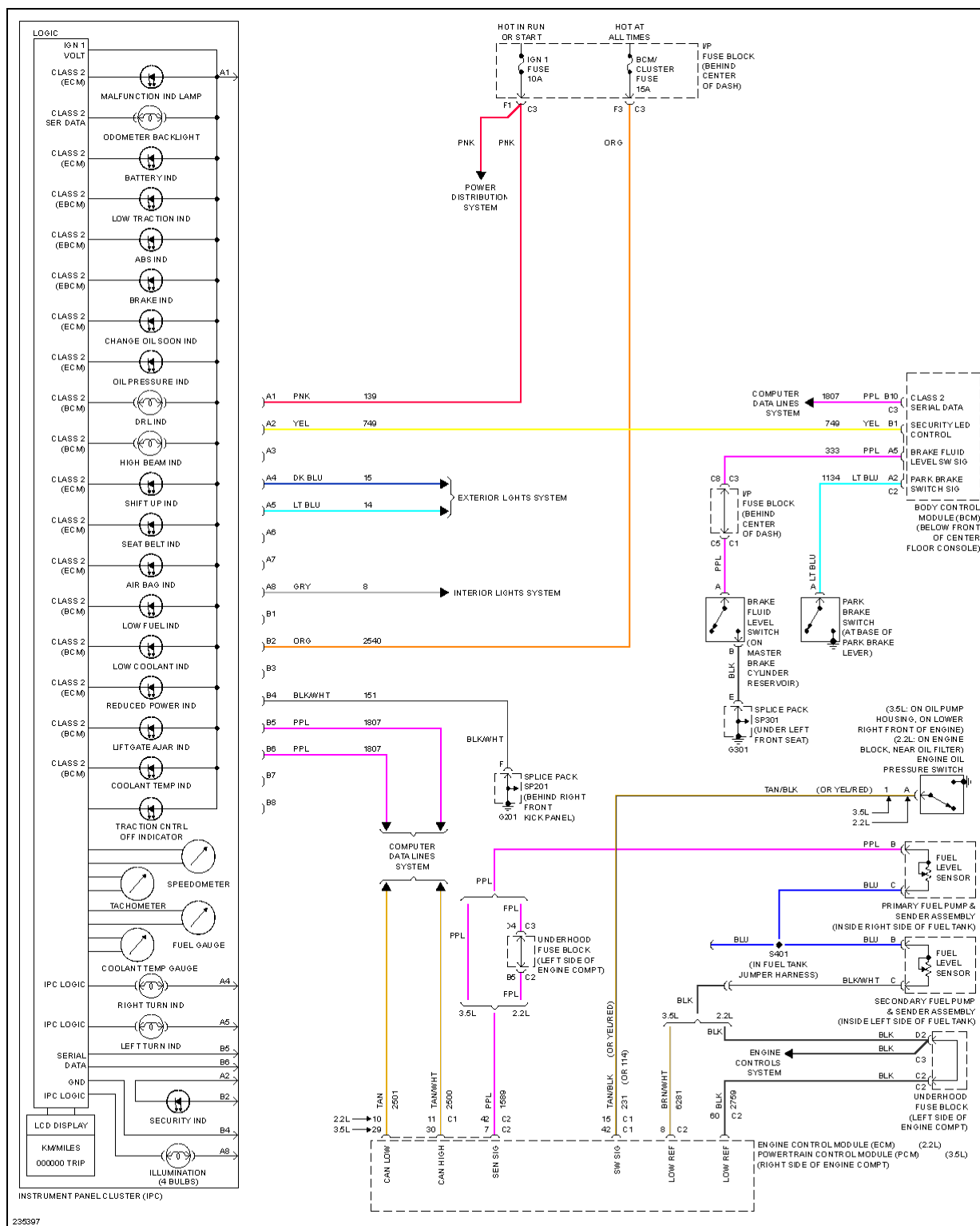
SYSTEM WIRING DIAGRAMS Fig. 35: Instrument Cluster Circuit
