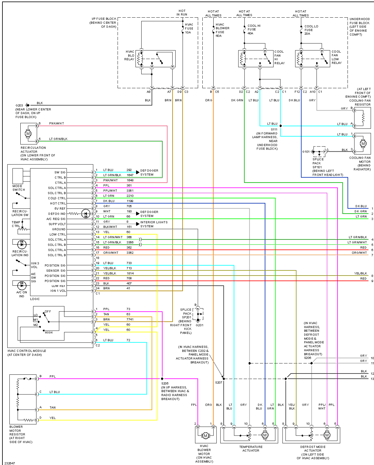
Fig. 2: 2.2L VIN D, Manual A/C Circuit (1 of 2)
