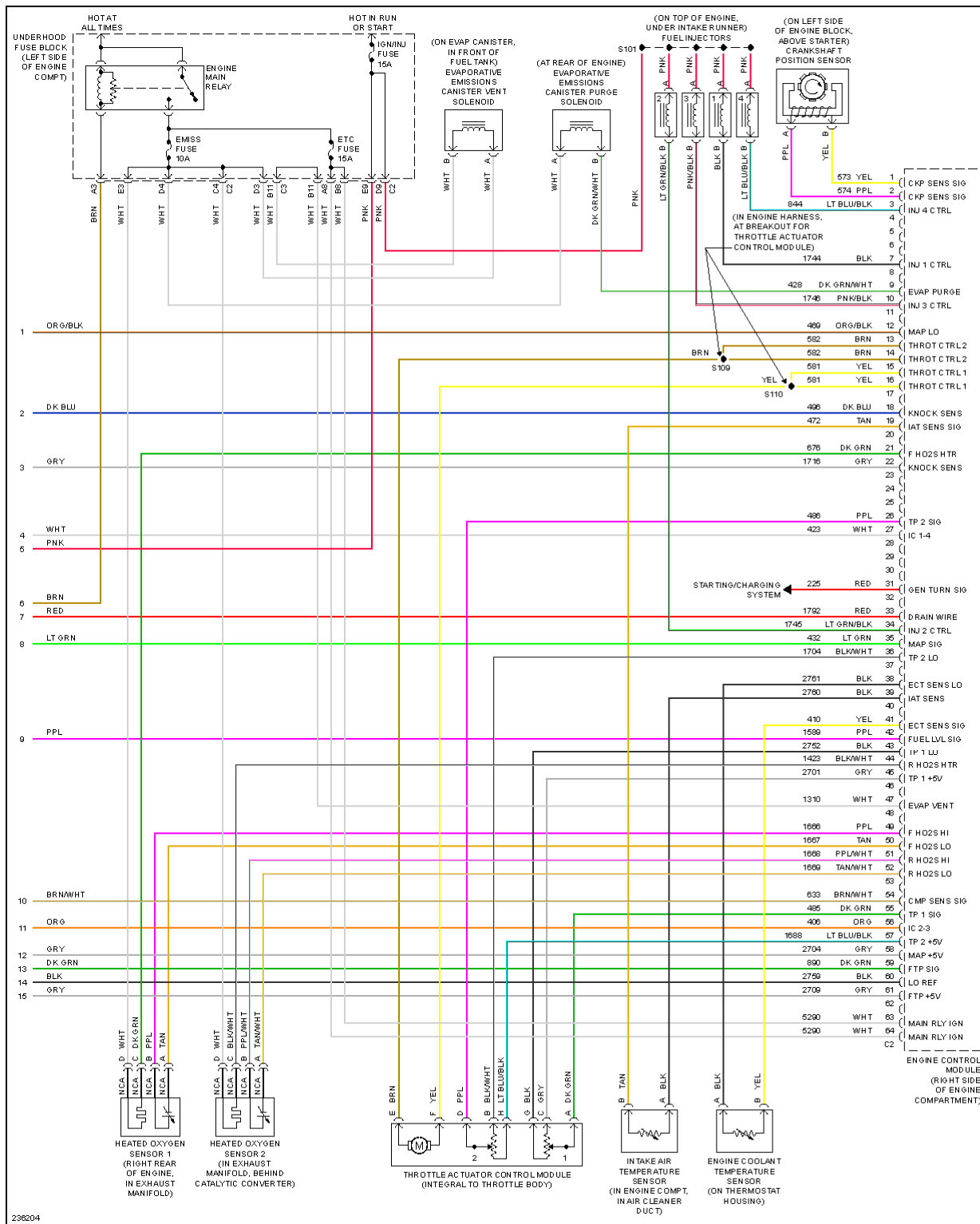
Fig. 20: 2.2L VIN D, Engine Performance Circuit (3 of 3)
