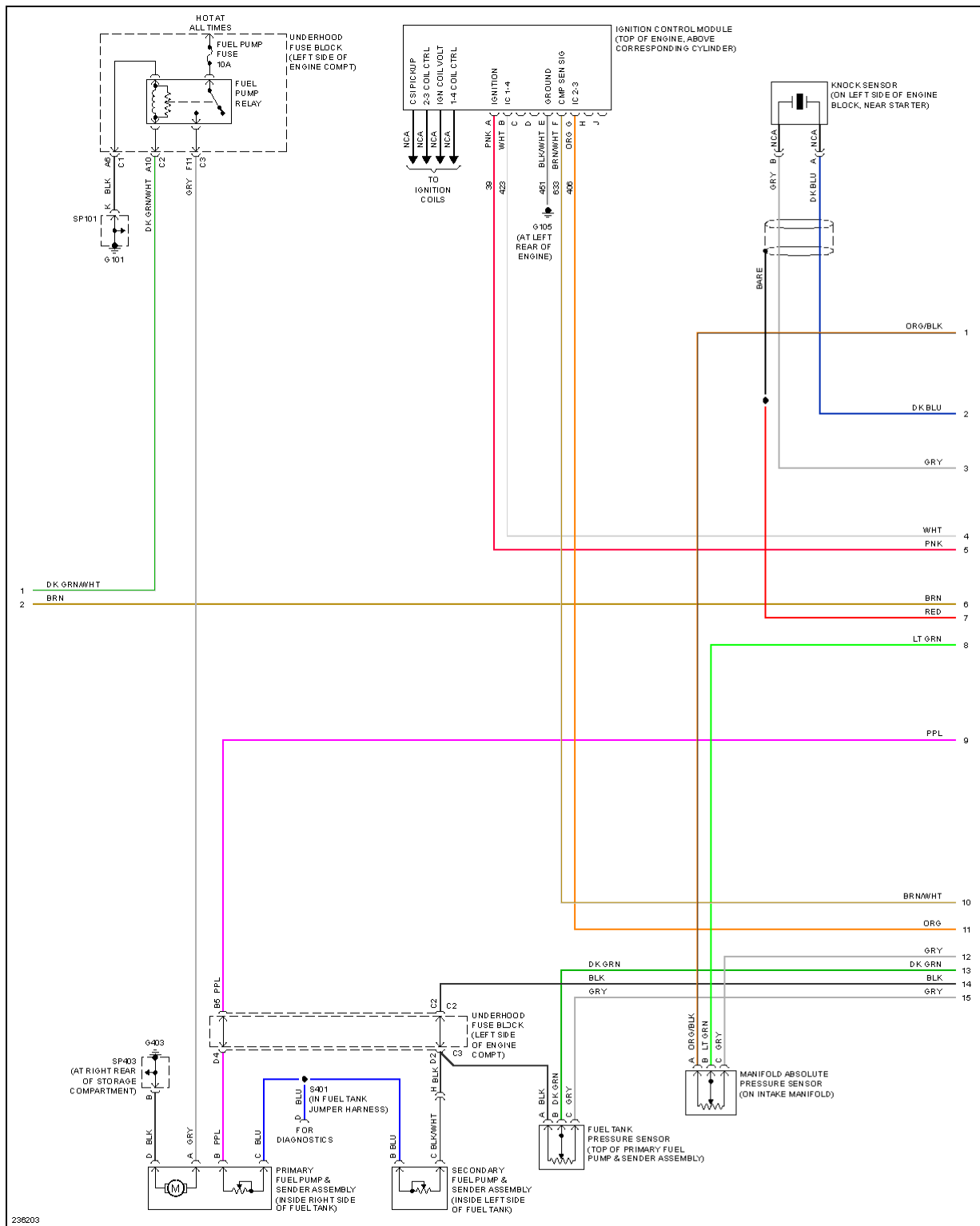
Fig. 19: 2.2L VIN D, Engine Performance Circuit (2 of 3)
