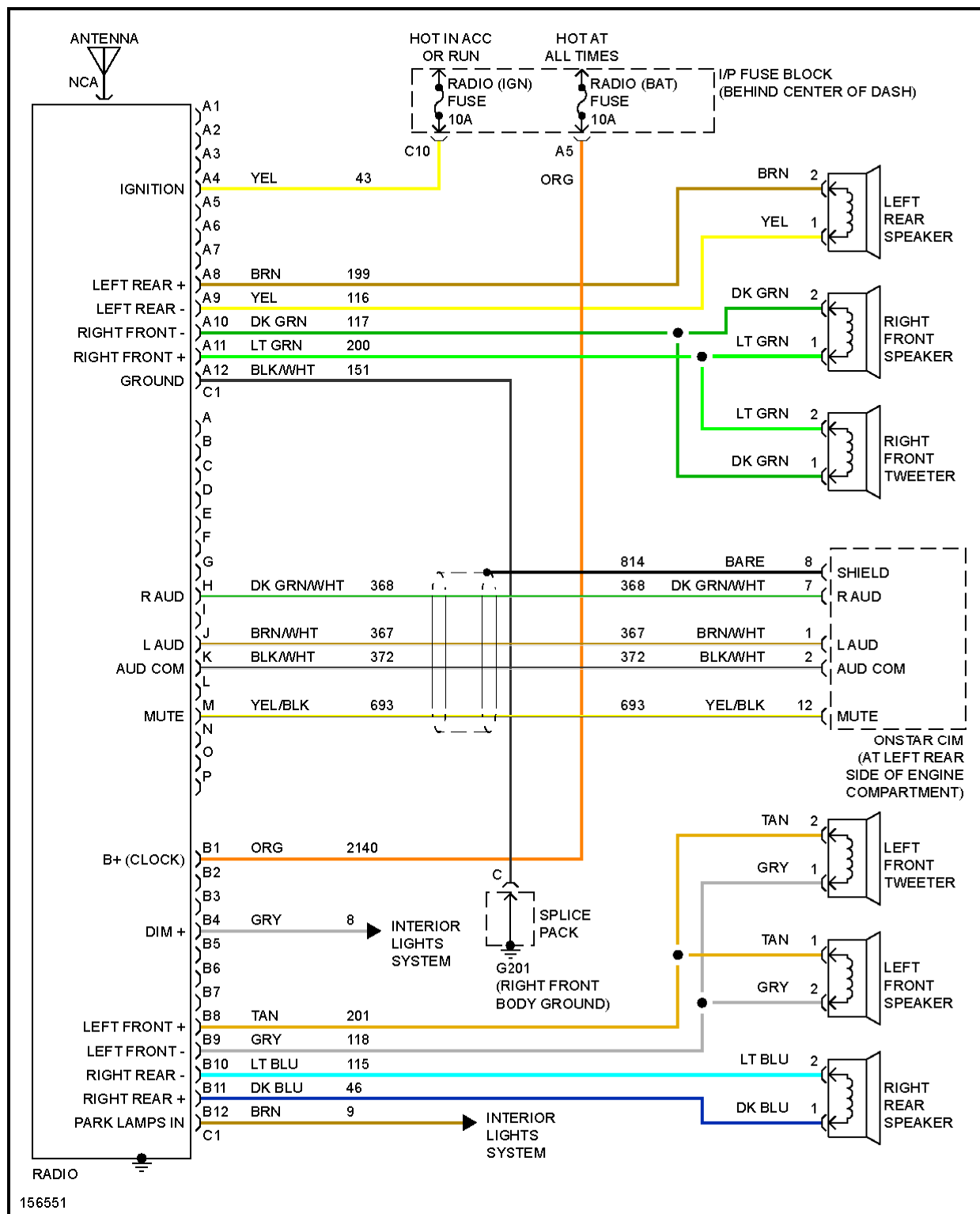
Fig. 47: Premium Sound Radio Circuit
