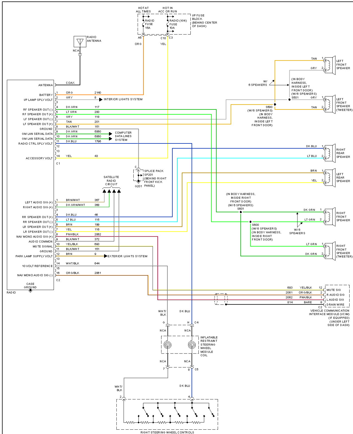
Fig. 53: Base Radio Circuit
