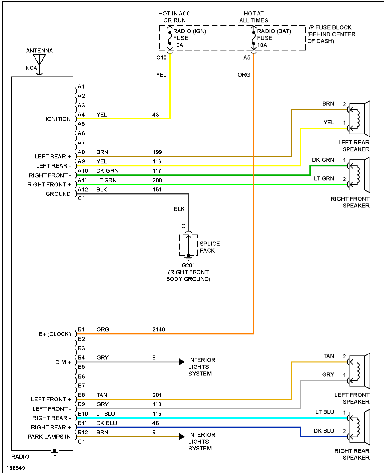
Fig. 46: Base Radio Circuit
