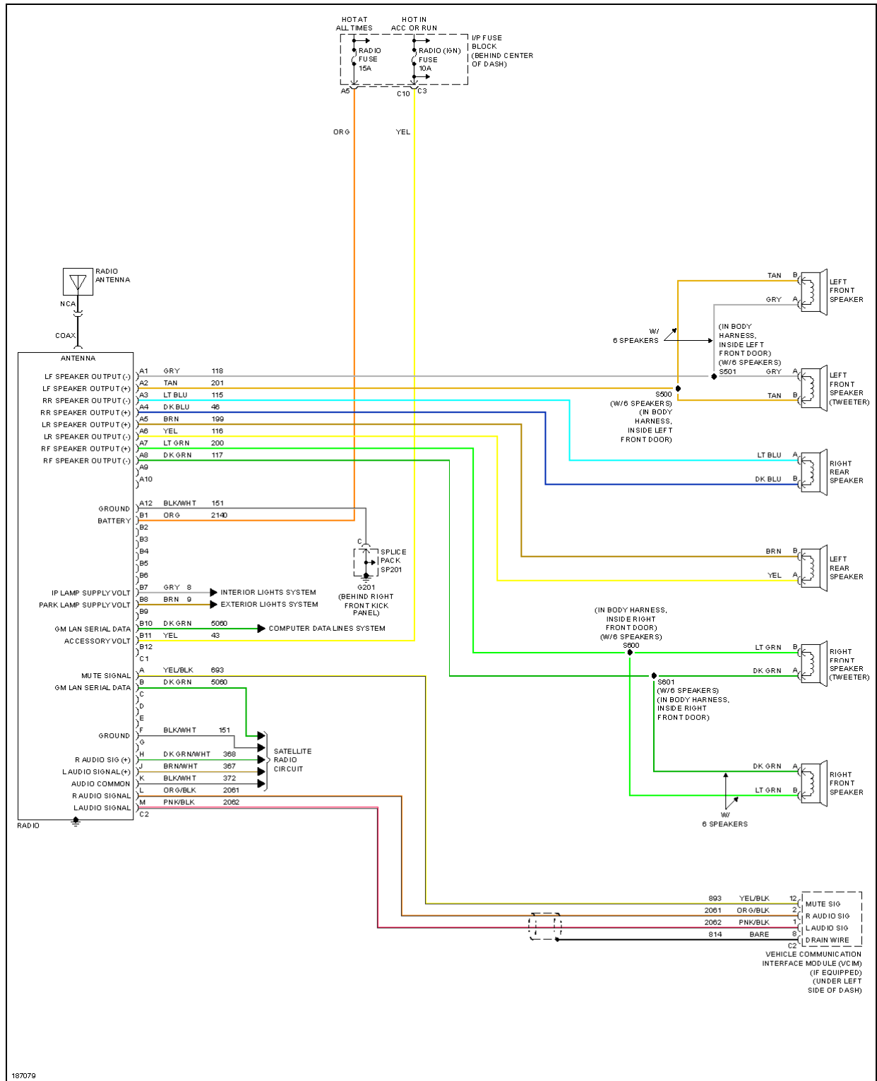
Fig. 57: Base Radio Circuit
